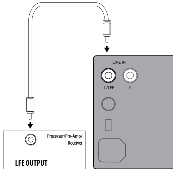
LFE Output on Processor/Pre-Amp/Receiver connected to LFE input on subwoofer amplifier
