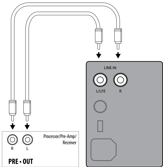
Left and Right pre-outs on Processor/Pre-Amp/Receiver connected to Left and Right line inputs on subwoofer amplifier
